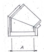
Schacht Bogen 45° EI60/Isol. 50mm
