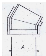
Schacht Bogen 15° EI60/Isol. 50mm
